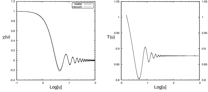
Figure A.3.1: ( Left panel ) Time evolution of the gravitational wave amplitude \chi(u) . Solid line represents a GW propagating in neutrino matter. Dashed line represents a GW propagating in vacuum. ( Right panel ) Time evolution of the transmitted wave intensity \mathcal{T} .
